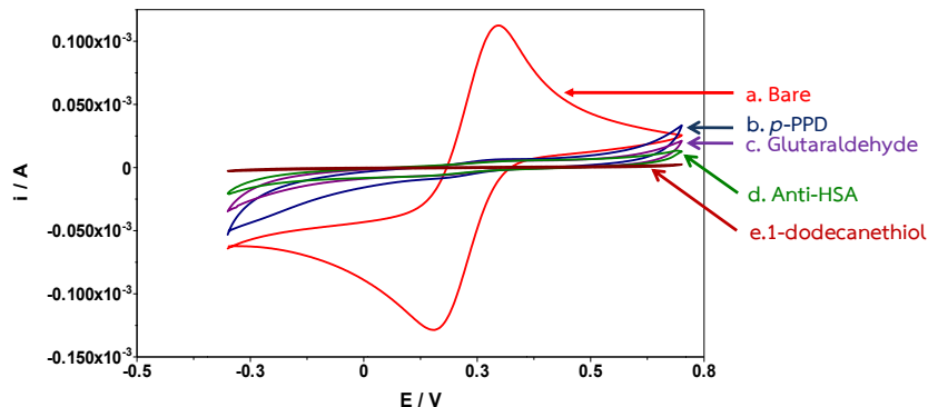
Figure 3 Cyclic voltammograms obtained from (a) bare gold, (b) PpPD, (c) glutaraldehyde, (d) anti-HSA and (e) blocking thiol, 1-dodecanethiol.
