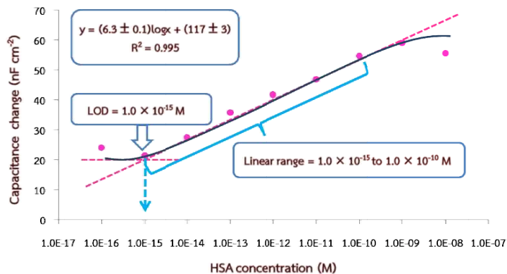
Figure 5 The calibration curve of HSA detection plotted between capacitance change and concentration.
