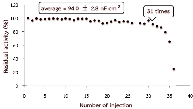
Figure 6 The residual activity and number of injection.
