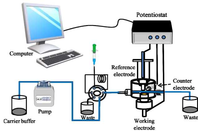
Figure 1 Schematic diagram showing an experimental setup of flow-injection immunosensor system.
