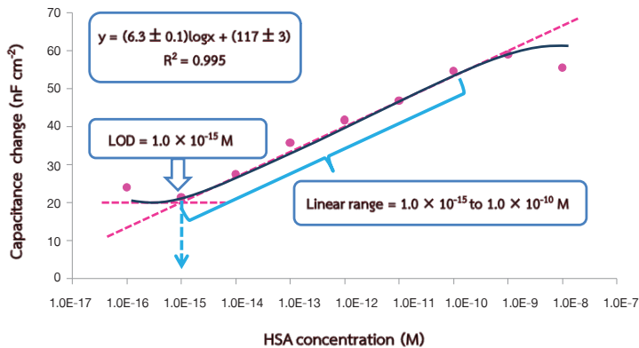
Figure 5 The calibration curve of HSA detection plotted between capacitance change and HSA concentration.
