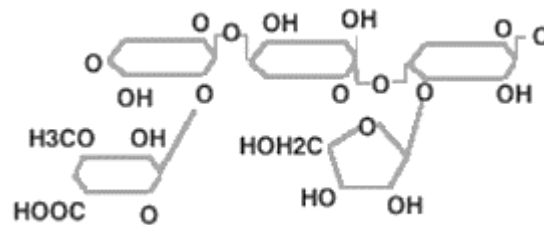
Figure 2 Hemicellulose Structure
