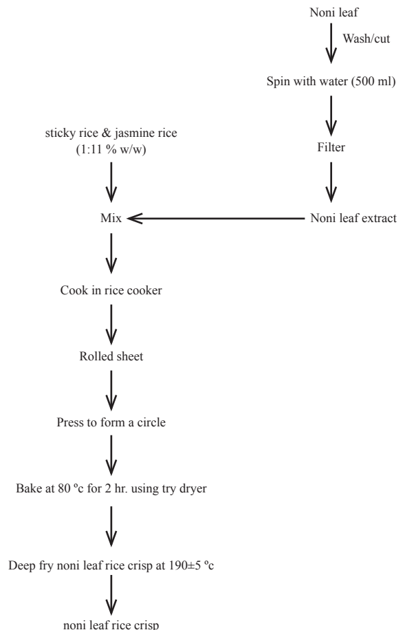
Fig.1 The production process of noni leaf rice crisp (modified from Techasiriwichai et al., 2015)
